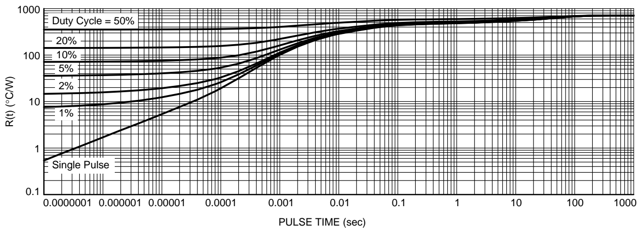
Figure 7. Thermal Response
